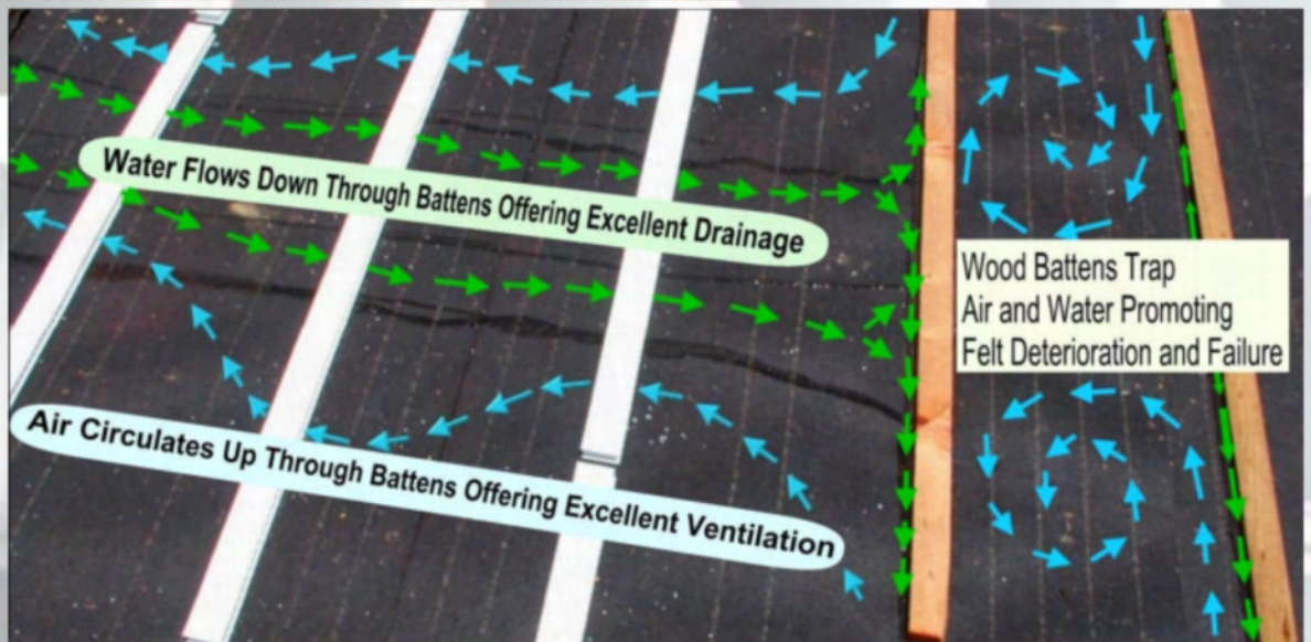
Felt Breakdown and Separation Caused By A Lack of Ventilation
