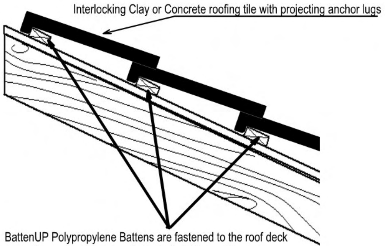
FIGURE 1 - TYPICAL SECTION
