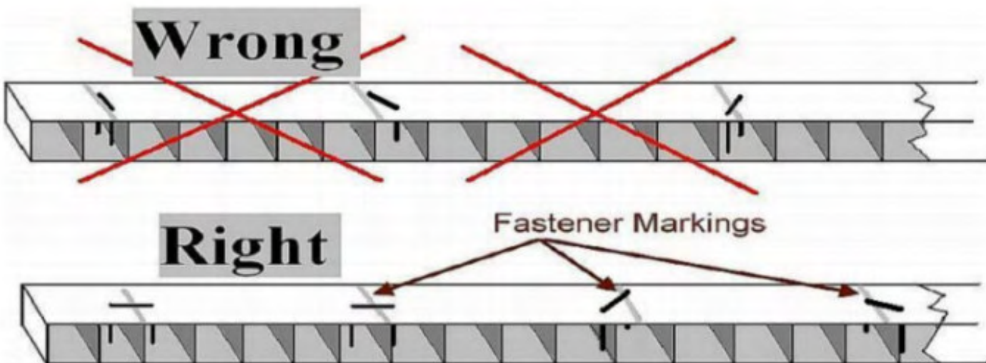
FIGURE 2 - FASTENING GUIDE - Stapes should straddle vertical partitions.
